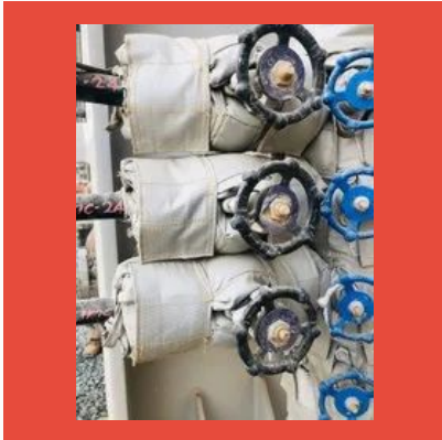
Removable and Reusable Insulation Jackets
